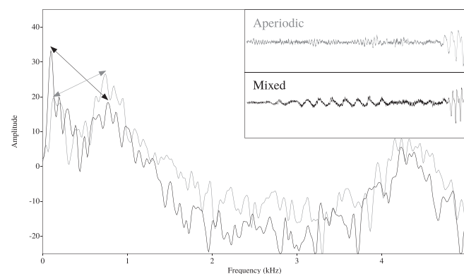
FIG. 4. Spectra from the middle 60 ms of aperiodic (gray) and mixed-source (black) dorsal fricatives in two repetitions of /Xut'ba/ by AF01. Arrows indicate amplitude peaks corresponding to source and filter components used to compute the SFR for each spectrum. Corresponding waveforms for the full consonant and initial periods of the following vowel are shown in the inset.
