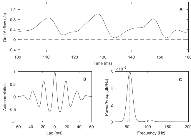
FIG. 2. Demonstration of the quantification of periodicity in oral airflow (A) via the autocorrelation function R_x (B) and the PSD of R_x (C). This sample is taken from the production of /Xu:n/ blood by PM01 in Fig. 1. The computed frequency of oscillation in this token (taken from Panel C) is 55 Hz.
