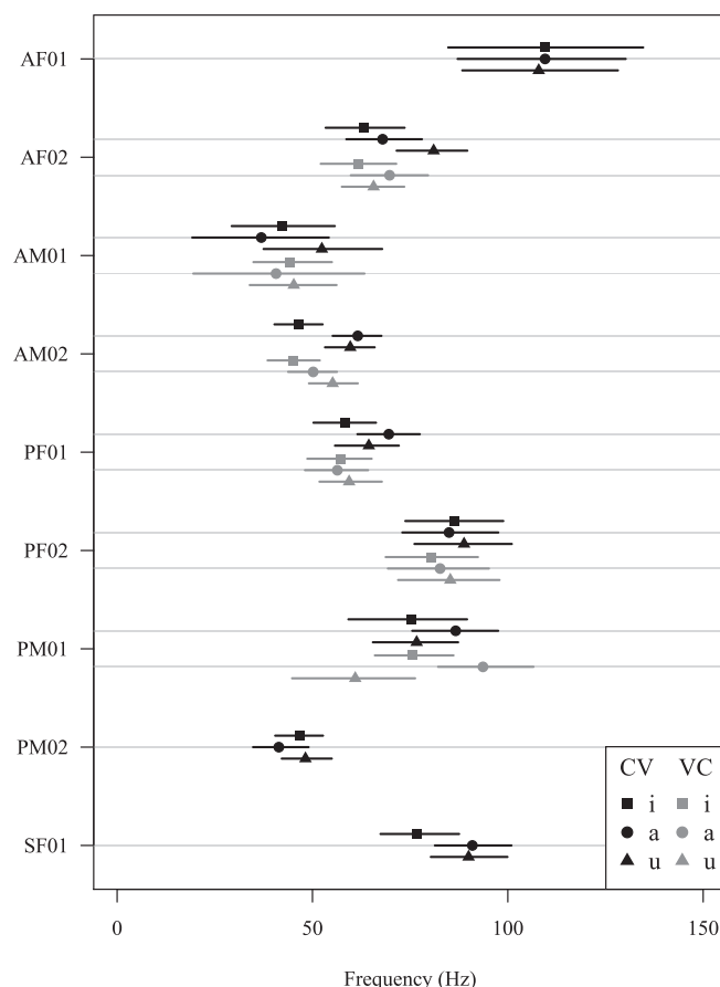
FIG. 3. Power-weighted mean frequency of oscillation in dorsal fricative airflow by speaker (vertical axis), position (CV, VC), and vowel context (i, a, u). Points represent medians of the posterior distribution in a Bayesian regression, with lines spanning the 95% credible interval (HPDI) over that distribution. Speakers SF02, SM01, and SM02 are not shown due to their sparse productions of mixed-source tokens, while AF01 and PM02 estimates are limited to CV position due to sparsity in mixed-source productions in VC position.
