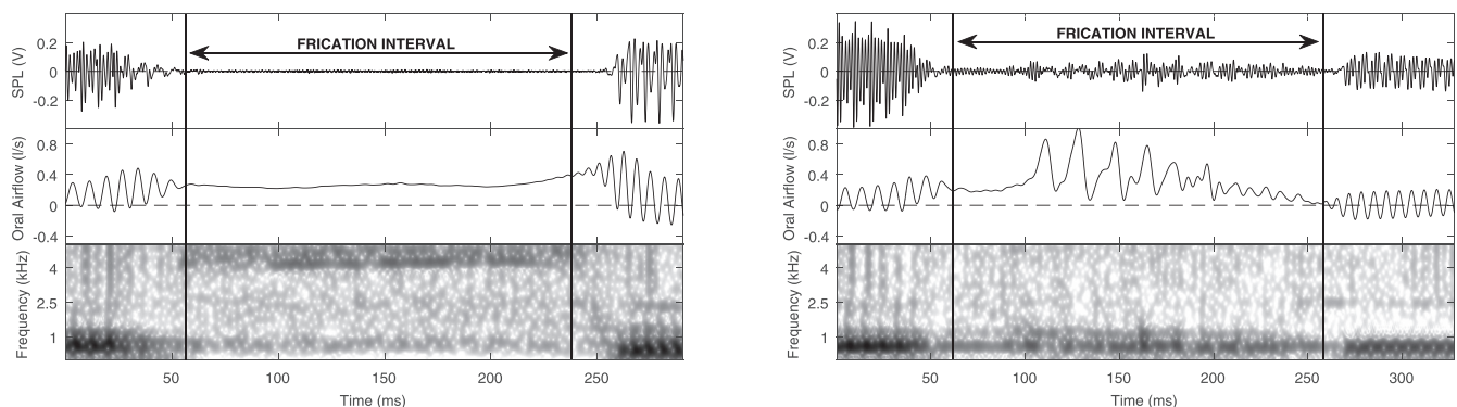
FIG. 1. Sample segmentation of the frication interval in the Persian words /sut/ “whistle” (left) and /Xu:n/ “blood” (right) by speaker PM01.
