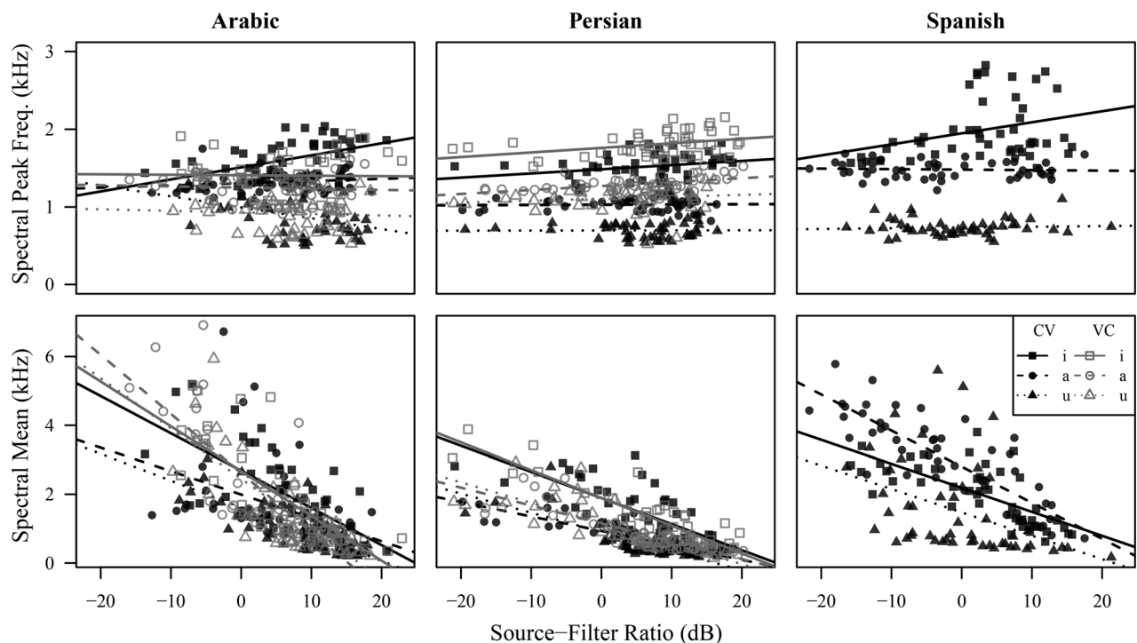
FIG. 5. Relationship between SFR and spectral peak frequency/spectral mean in Arabic, Persian, and Spanish.
